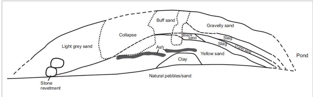
Figure 1 – Schematic section of east face of dam
