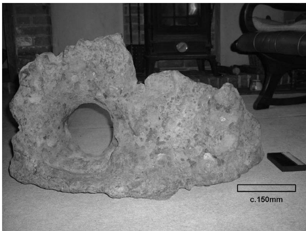
Figure 1: Iron mass from near Beckley Furnace, East Sussex
