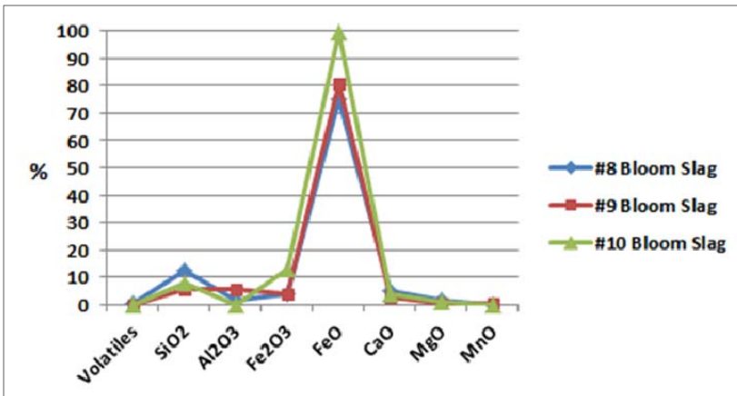
Figure 5 – Comparison of Bloom Slags Mineral Contents
