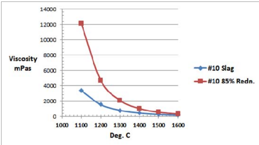
Figure 8 – Viscosities for smelt 10 Cinder Slag before and after 85% Reduction
