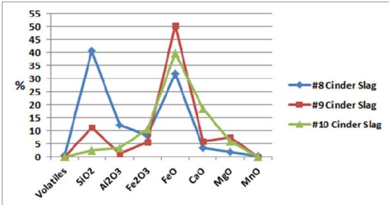
Figure 4 – Comparing Sample Cinder Slag Mineral Profiles
